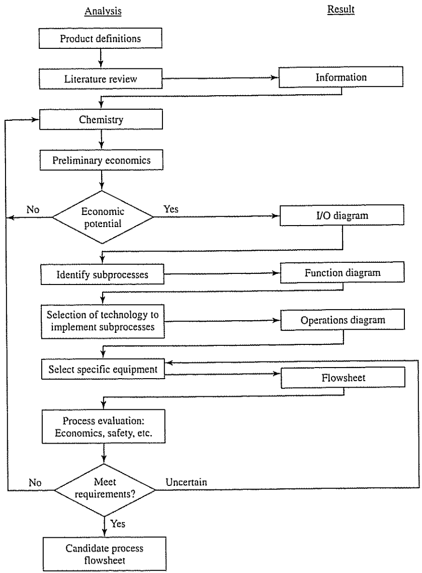
Figure 4-1 Flow diagram illustrating hierarchical process—flowsheet synthesis, development, evaluation, and selection
