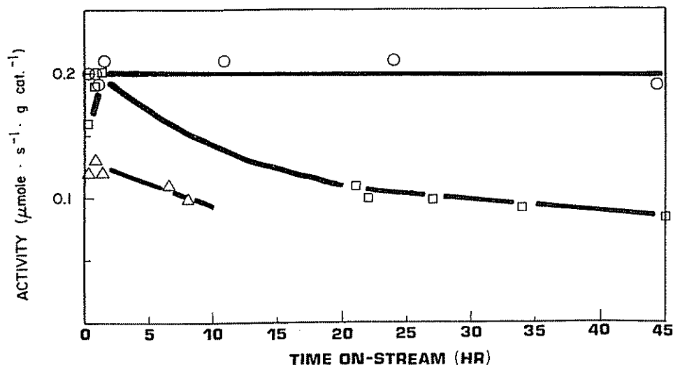
FIG. 1. Rate of \text{CH}_4 formation as a function of time on-stream. P = 101 \text{ kPa} , T = 508 \text{ K} , \text{H}_2/\text{CO} = 3 : \circ , 5.0% Fe/C-1; \triangle , 4.5% Fe/V3G; \square , 10% Fe/ \text{Al}_2\text{O}_3 .
