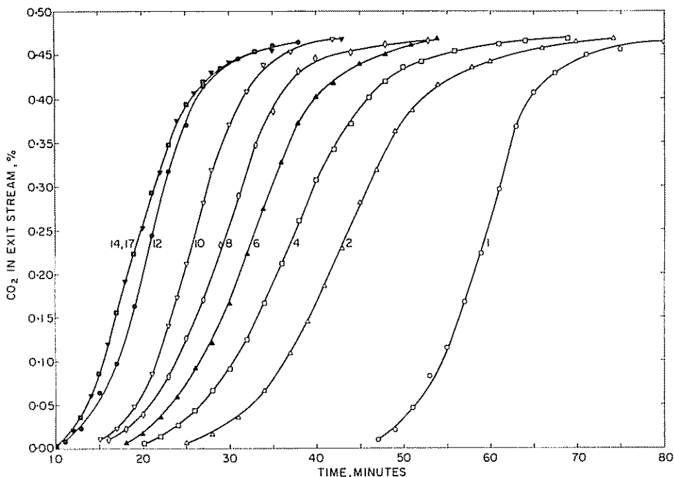
Fig. 7. Effect of recycling on the break through curves of dry \text{CO}_2 at 25^\circ\text{C} on active carbon, originally outgassed at 900^\circ\text{C} .
