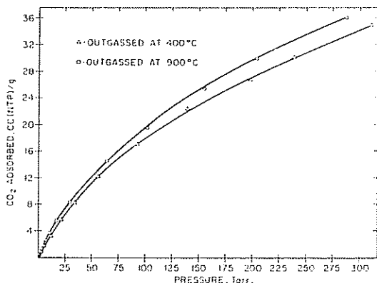
Fig. 10. Effect of outgassing temperature on sorption isotherms of CO 2 on CMS-B at 25°C.
