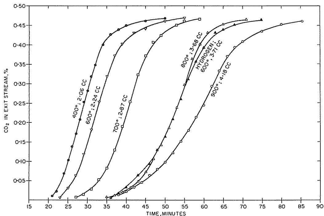
Fig. 6. Effect of heat treatment in He and H 2 at different temperatures on the break through curves of dry CO 2 at 25°C on active carbon. Value given for each curve is total uptake per gram of adsorbent.
