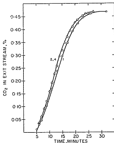
Fig. 9. Effect of recycling on the break through curves of dry \text{CO}_2 at 25°C on de-ashed carbon originally outgassed at 900°C.
