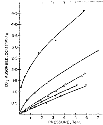
Fig. 3. Sorption isotherms of CO 2 on active carbon and carbon sieves in low pressure region at 25°C. As-received active carbon outgassed at 400°C, O; 900°C, ●; De-ashed active carbon outgassed at 400°C, ∇; 900°C, ▼; CMS-A, □, and CMS-B, Δ, degassed at 400°C.
