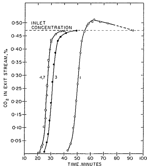
Fig. 8. Effect of recycling on the break through curves of wet \text{CO}_2 at 25^\circ\text{C} on active carbon, originally outgassed at 900^\circ\text{C} .
