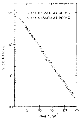
Fig. 4. Dubinin plots for CO 2 adsorption on CMS-B at 25°C.
