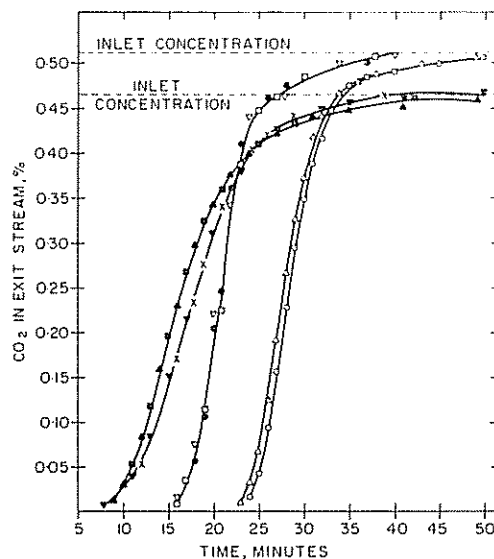
Fig. 1. Effect of recycling on the break through curves of dry \text{CO}_2 at 25^\circ\text{C} on active carbon and carbon sieves, originally outgassed at 400^\circ\text{C} . Active carbon: cycle 1, \circ ; 2, \triangle ; 3, \square ; 6, \nabla ; 7, \bullet . CMS-A: cycle 1, \nabla ; 2, \times . CMS-B: Cycle 1, \triangle ; 2, \square .
