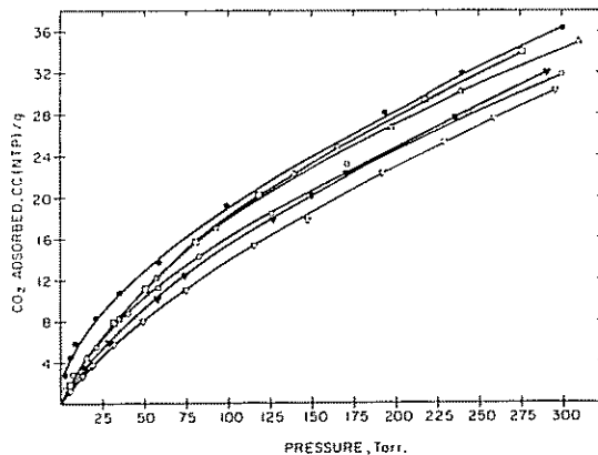
Fig. 2. Sorption isotherms of CO 2 on active carbon and carbon sieves at 25°C. As-received active carbon outgassed at 400°C, O; 900°C, ●; De-ashed active carbon outgassed at 400°C, ∇; 900°C, ▼; CMS-A, □; and CMS-B, Δ, degassed at 400°C.
