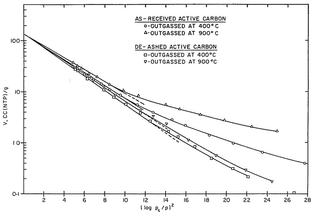
Fig. 5. Dubinin plots for \text{CO}_2 adsorption on active carbon at 25^\circ\text{C} .
