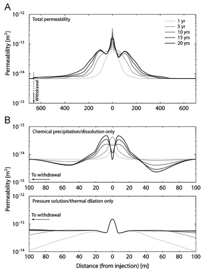
Fig. 5. Permeability changes using water #2: (A) total permeability change with distance from injection and (B) mineral precipitation/dissolution portion and thermal-hydraulic portion of total permeability change in (A). Note the change of scale on the x-axis of (B).
