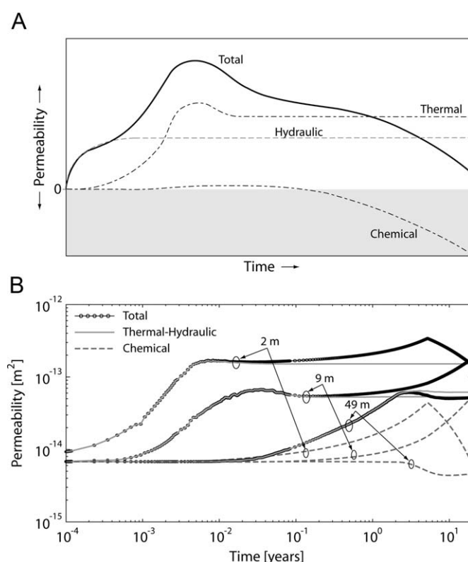
Fig. 3. (A) Conceptual model of permeability altering processes after [26] and (B) contribution of each mechanism to total permeability change in our simulations. Analogous to (A). Changes monitored at 2, 9, and 49 m from injection. Uses water #2.
