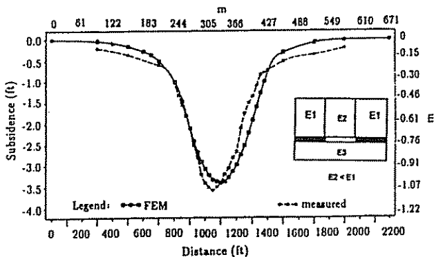
Fig. 15. Comparison of calculated and measured subsidence (b)
