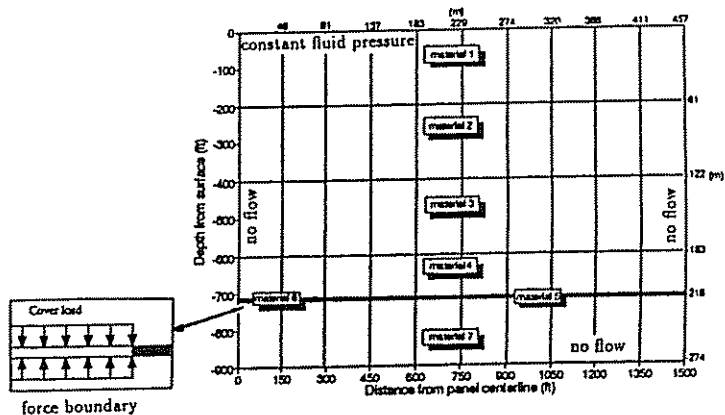
Fig. 10. Finite element layout
