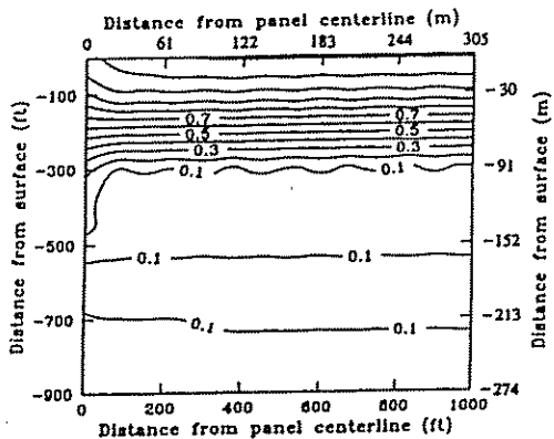
Fig. 7. Normalized pre-mining hydraulic conductivity
