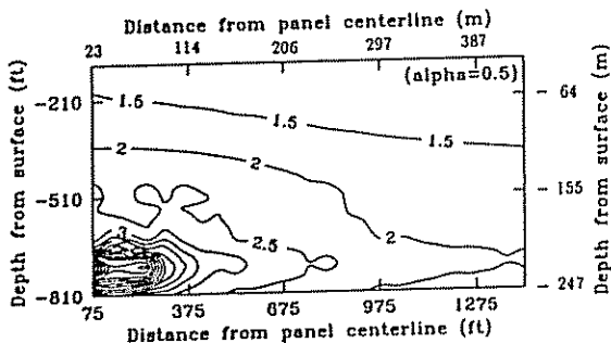
Fig. 16. Ratio of conductivity ( K/K_0 ) in intact rock ( \alpha = 0.5 )
