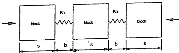
Fig. 4. A simple fracture-block mechanism, ( s ) spacing, ( b ) aperture, ( K_n ) fracture stiffness
