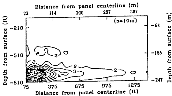
Fig. 18. Ratio of conductivity ( K/K_0 ) in fractured rock ( s = 10\text{ m} )
