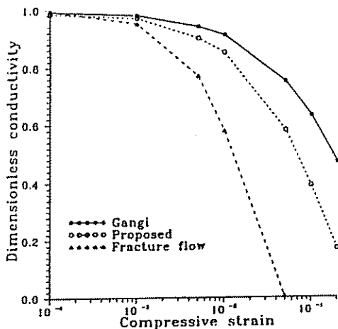
Fig. 5. Compressive strain versus dimensionless conductivity
