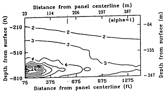
Fig. 17. Ratio of conductivity ( K/K_0 ) in intact rock ( \alpha = 1.0 )
