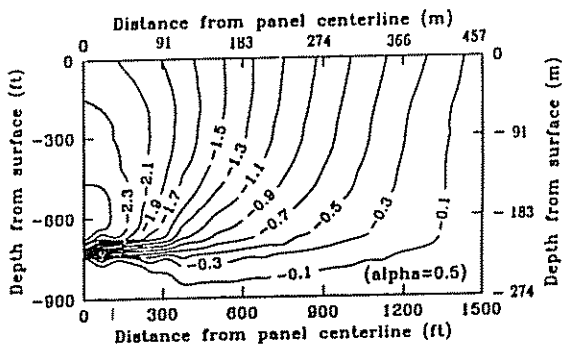
Fig. 11. Subsidence contour ( \alpha = 0.5 )
