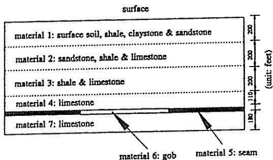
Fig. 8. Strata lithology over a panel
