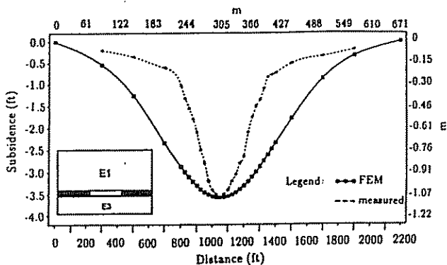
Fig. 14. Comparison of calculated and measured subsidence (a)
