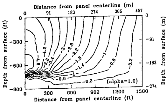
Fig. 12. Subsidence contour ( \alpha = 1.0 )
