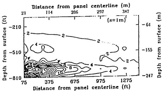
Fig. 19. Ratio of conductivity ( K/K_0 ) in fractured rock ( s = 1\text{ m} )
