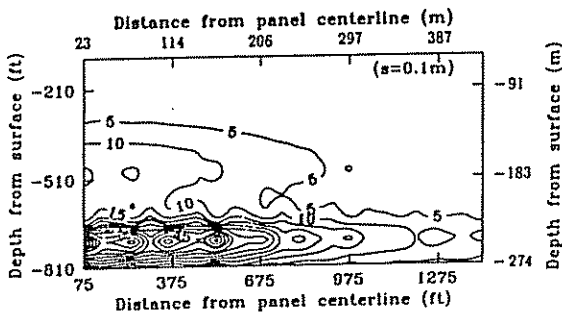
Fig. 20. Ratio of conductivity ( K/K_0 ) in fractured rock ( s = 0.1\text{ m} )
