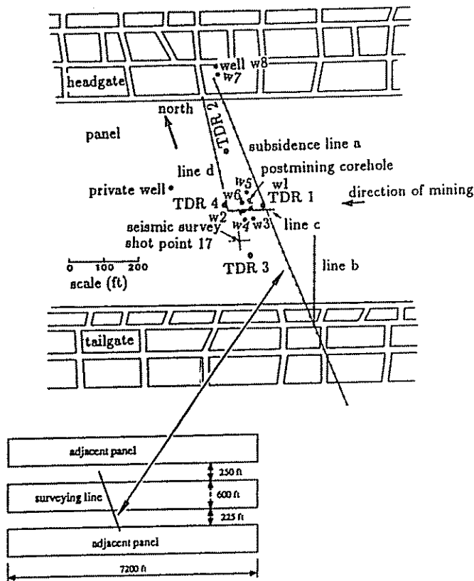
Fig. 9. Layout of mine panels
