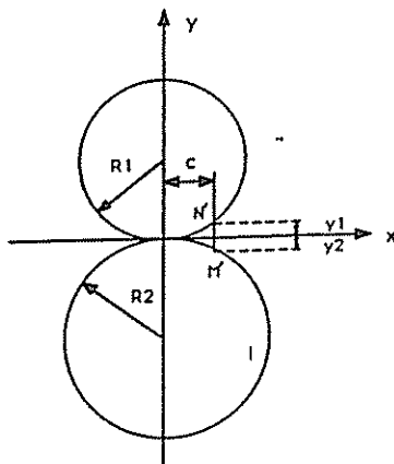
Fig. 2. Configuration of spherical contact
