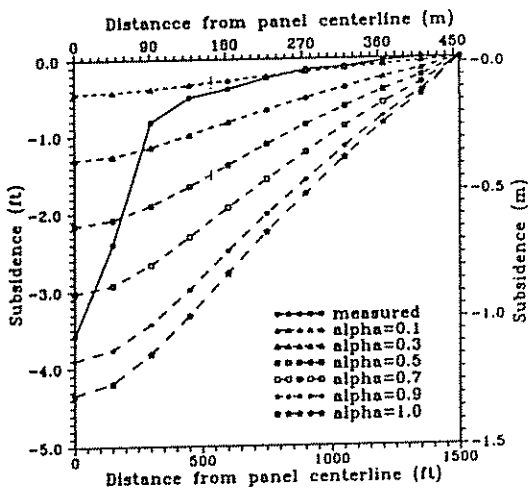
Fig. 13. Measured and calculated subsidence with various \alpha
