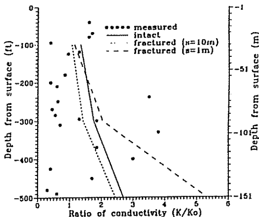
Fig. 22. Ratio of conductivity between models and measurement.
