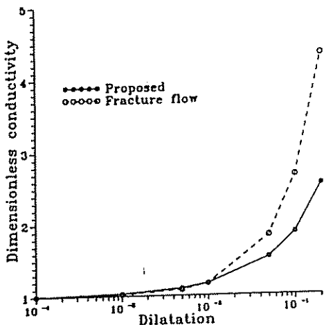
Fig. 6. Dilatation versus dimensionless conductivity
