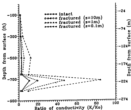
Fig. 21. Ratio of conductivity close to panel centerline
