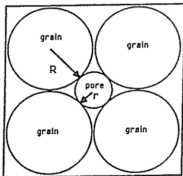
Fig. 1. Cubical packing of grains
