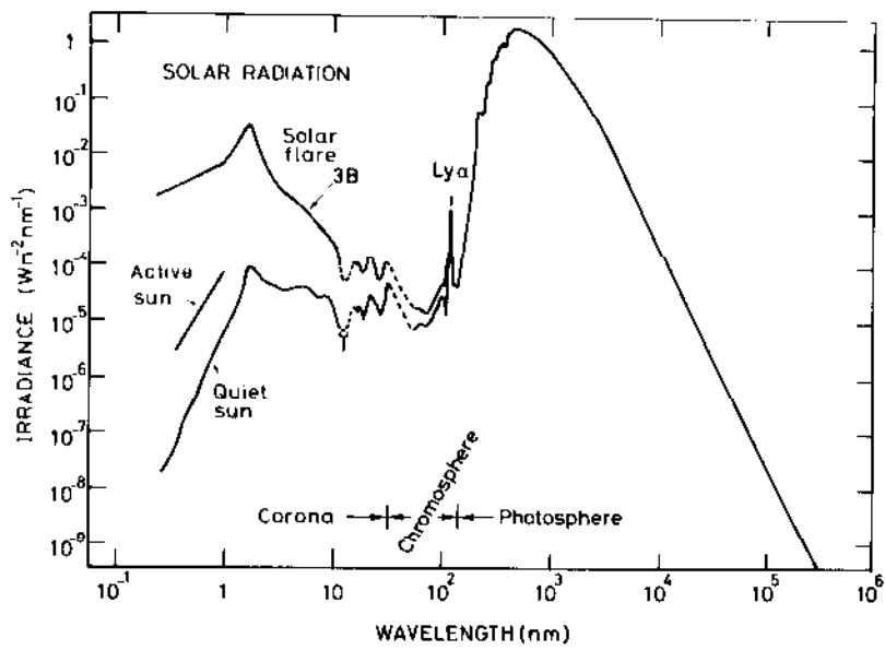
Fig. 4.5. Spectral distribution of the solar irradiance, and its variation with solar activity. The logarithmic representation emphasizes the contribution of x-rays and extreme ultraviolet radiation. After Smith and Gottlieb (1974).
