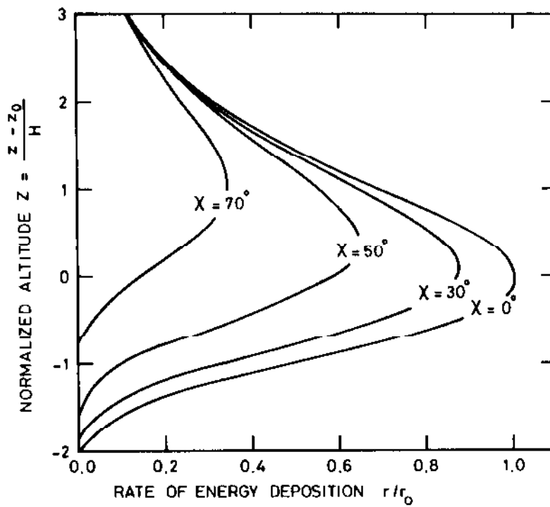
Fig. 4.10. Appearance of a characteristic layer due to absorption of solar energy. Distribution obtained by Chapman theory for different values of the zenith angle.
